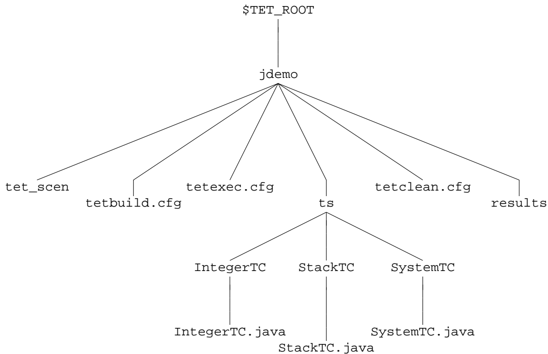
Figure 20. Directory structure for the Java demonstration test suite
